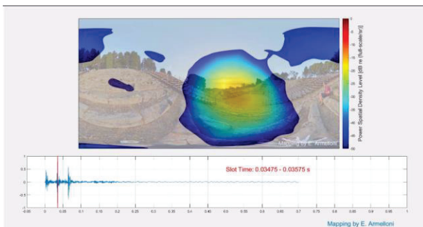
Figure 12. Acoustical map showing the energy of first reflection, source S1 is directed towards the skené.
