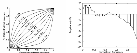
Fig. 1. Bilinear transformation of frequency with different \lambda values (left), SPL shape of a target environment (right).
