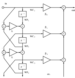
Fig. 3. WFIR filter structure.
