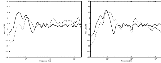
Fig. 4. Frequency response with 350 FIR equalization (solid line) and without (dashed line), Citroën Evasion cockpit, left channel (left), right channel (right)
